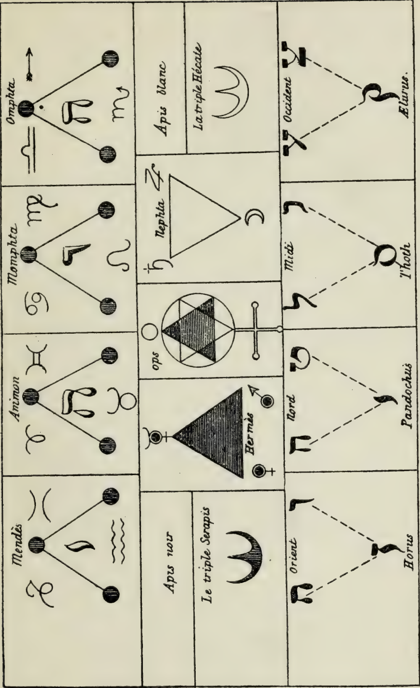
EXPLANATORY DIAGRAM OF THE ASTRONOMICAL AND ALPHABETICAL TABLET OF BEMBO
